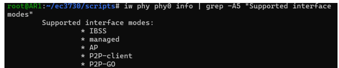
Fig. 30. Supported wireless interface modes reported by the Raspberry Pi 5 Broadcom wireless chipset. The absence of IEEE 802.11s mesh-point support prevented native wireless mesh operation.
